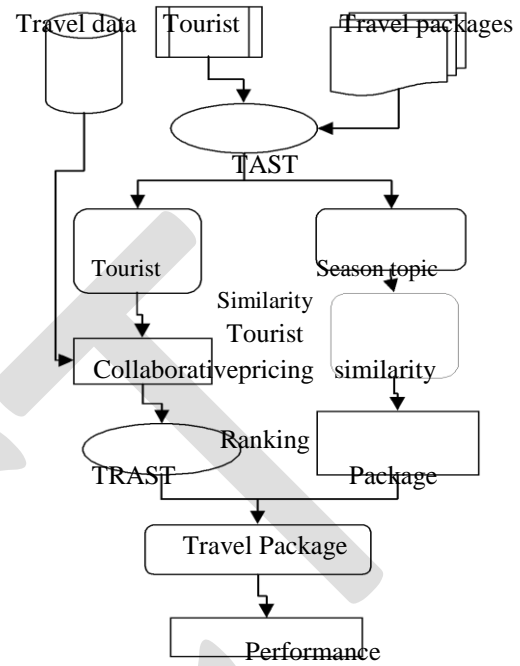
Fig 1: System Architecture
