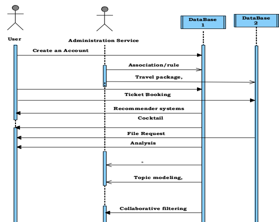
Fig 3: Sequence Diagram
